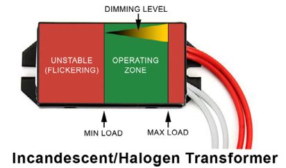
Incandescent/Halogen Transformer
